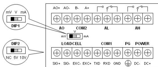
Signal Terminal
